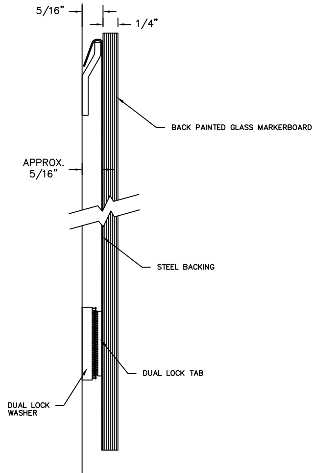
SECTION "A-A"
