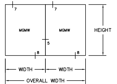
TYPICAL ELEVATION NTS
